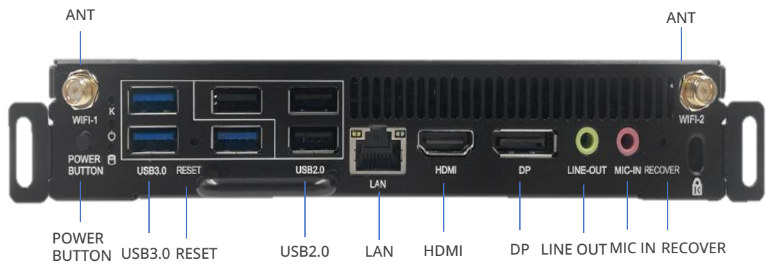
FRONT
